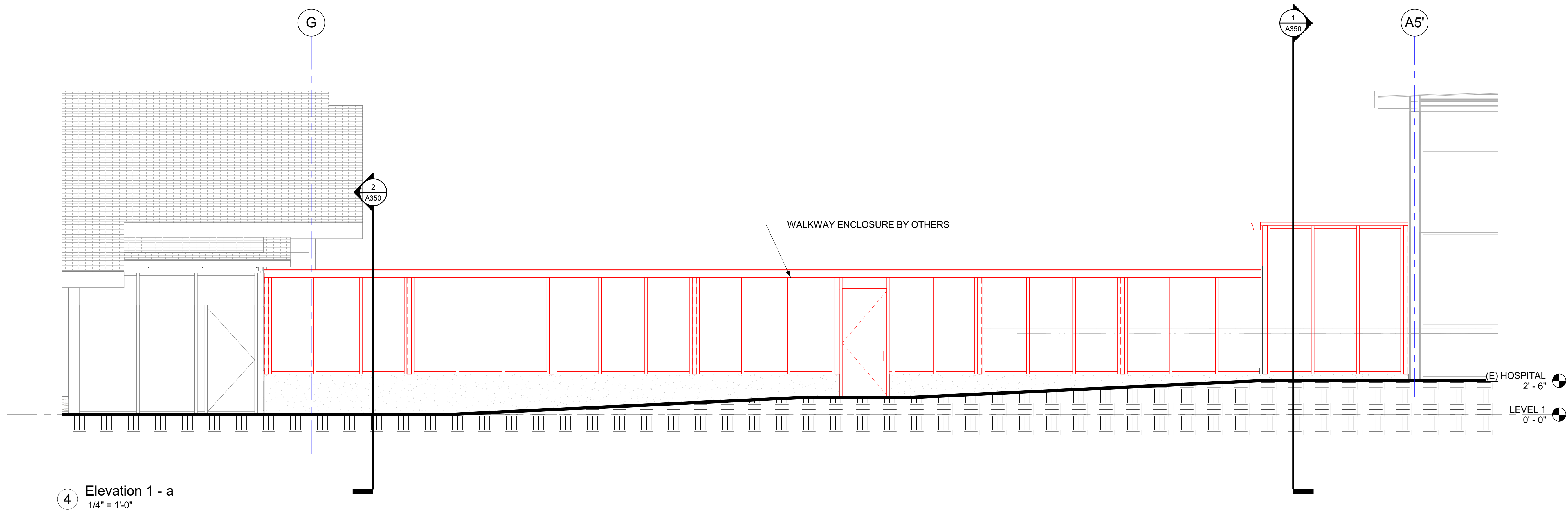
3 MEDICAL OFFICE BUILDING EAST WEST SECTION 1/4" = 1'-0"
