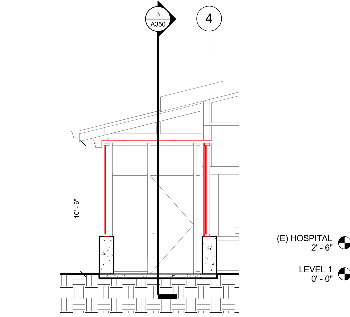
2 SECTION AT MOB 1/4" = 1'-0"
