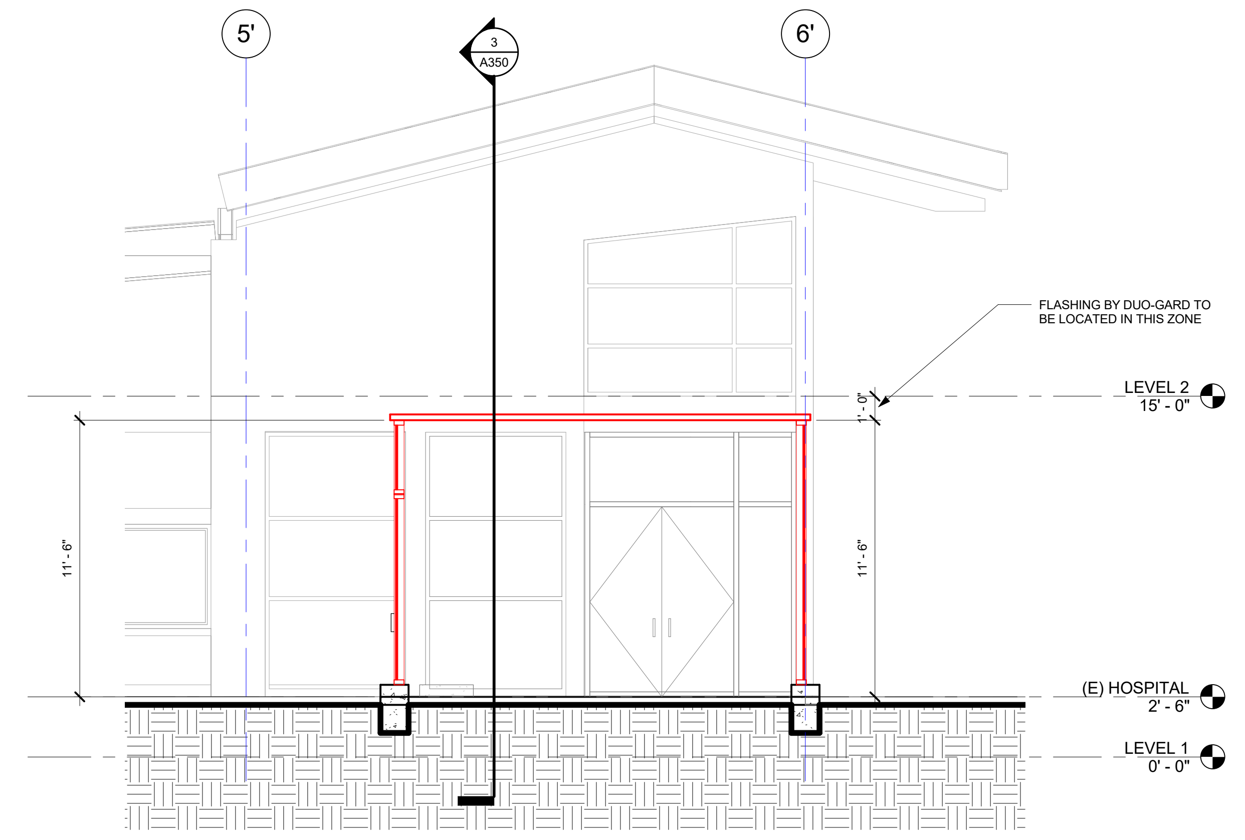
1 SECTION AT HOSPITAL 1/4" = 1'-0"
